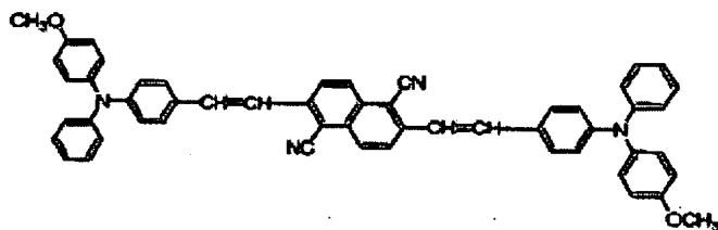
Structural formula (17)-1:
